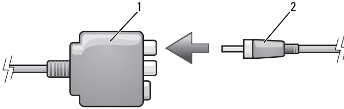
1 composietvideo-adapter 2 S/DPDIF digitale audiokabel
